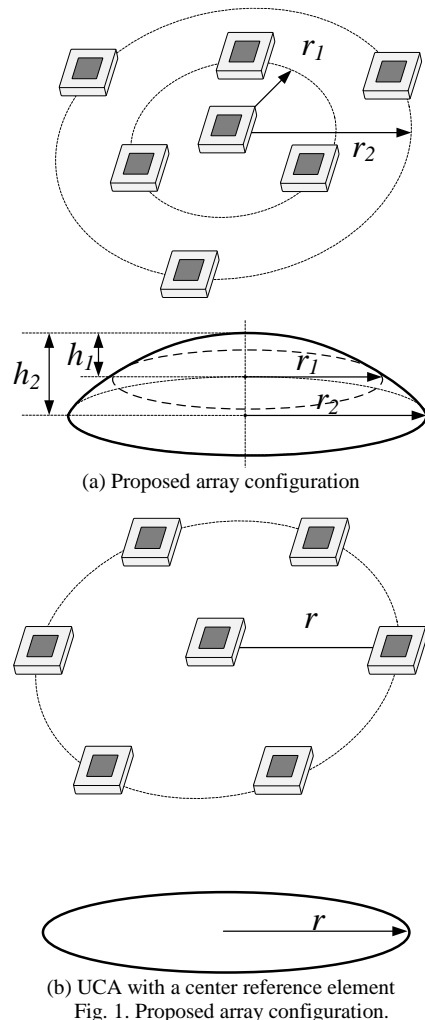
Fig. 1. Proposed array configuration.
